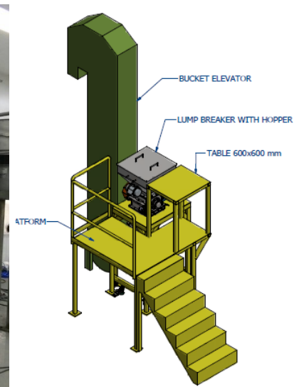
Complete station with Control panel with frequency inverter, Low loading hopper and top cover, Metal base with wheel and lockable stand, Operation platform, Bag laying table, Hand rail and Stair
